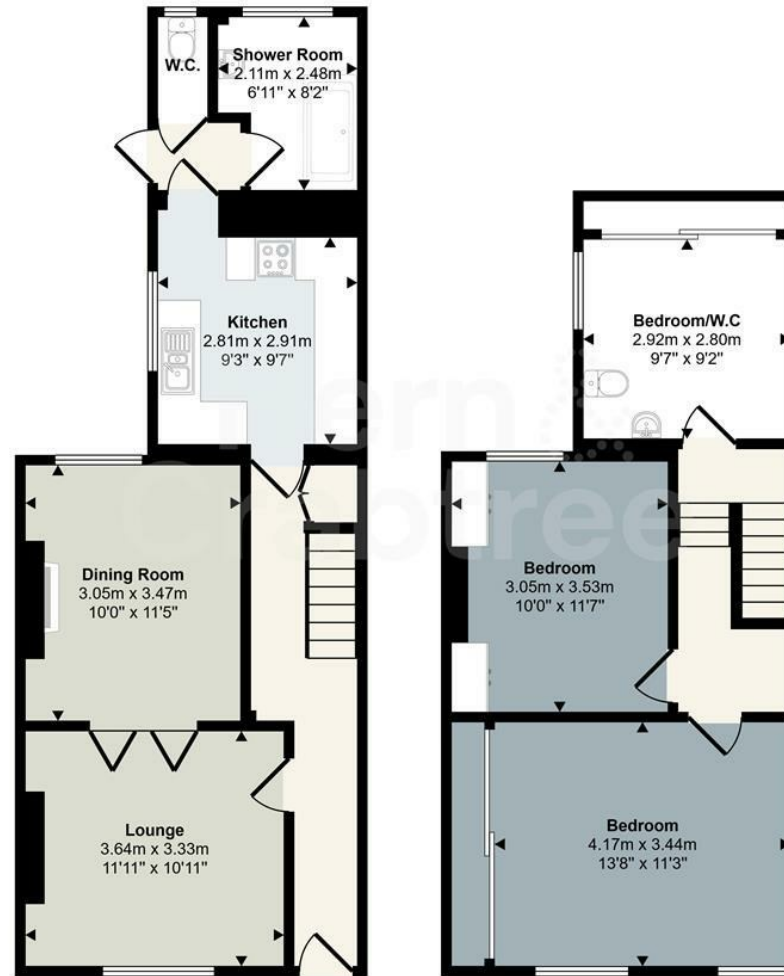
Ground Floor Approx 52 sq m / 557 sq ft
